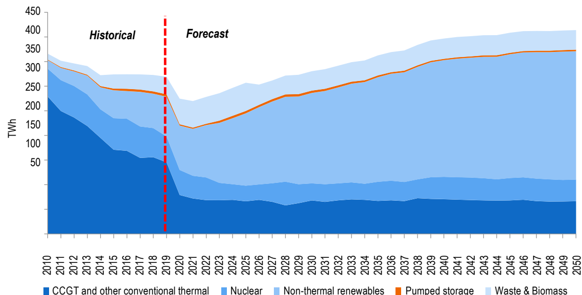
UK Electricity Generation Overview
