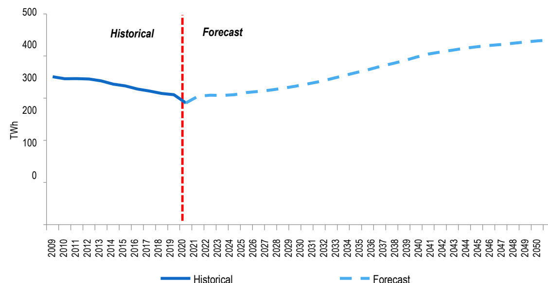
UK Electricity Demand Overview
